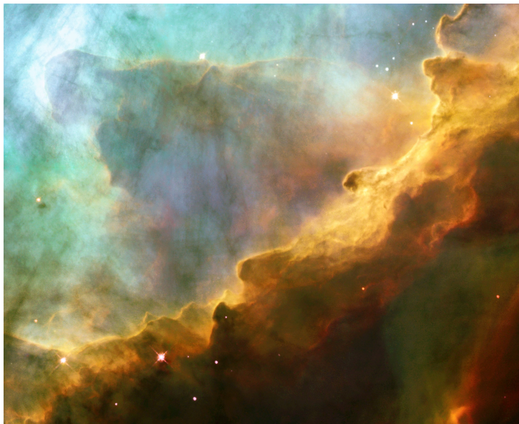
Omega Nebula
